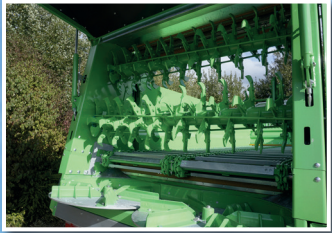
2 horizontal beaters with spreading table (2 x ø 1,040 mm)
